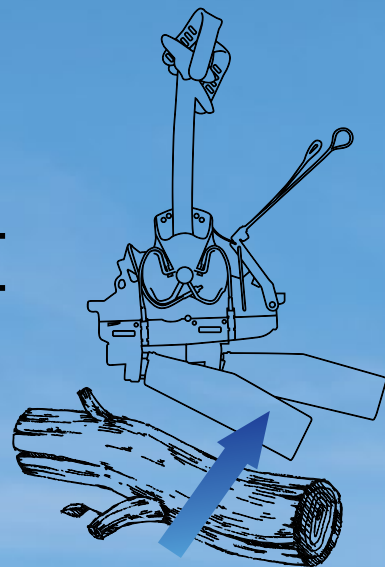
Kick-up Fins Retract When Impacting an Underwater Obstacle
